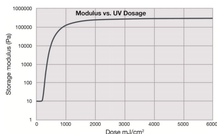
Figure 1: Storage modulus vs. UV dosage
